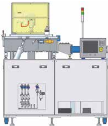
大尺寸面板的光阻去除設備 Panel type PR removal system
